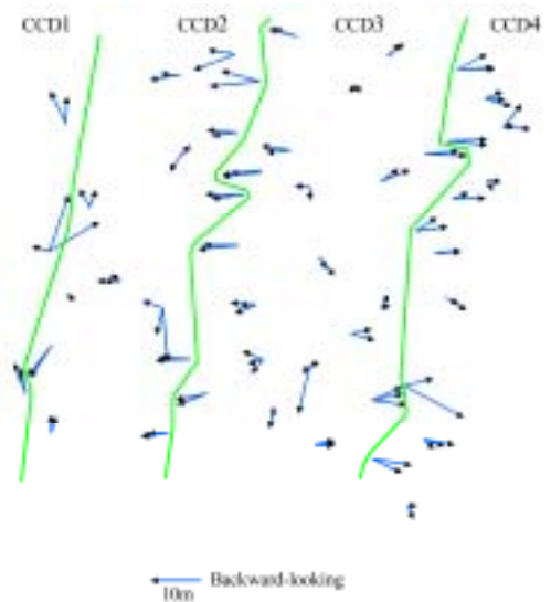
Fig. 7 Residuals of image observation (adjustment of rotation of the radiometers)
