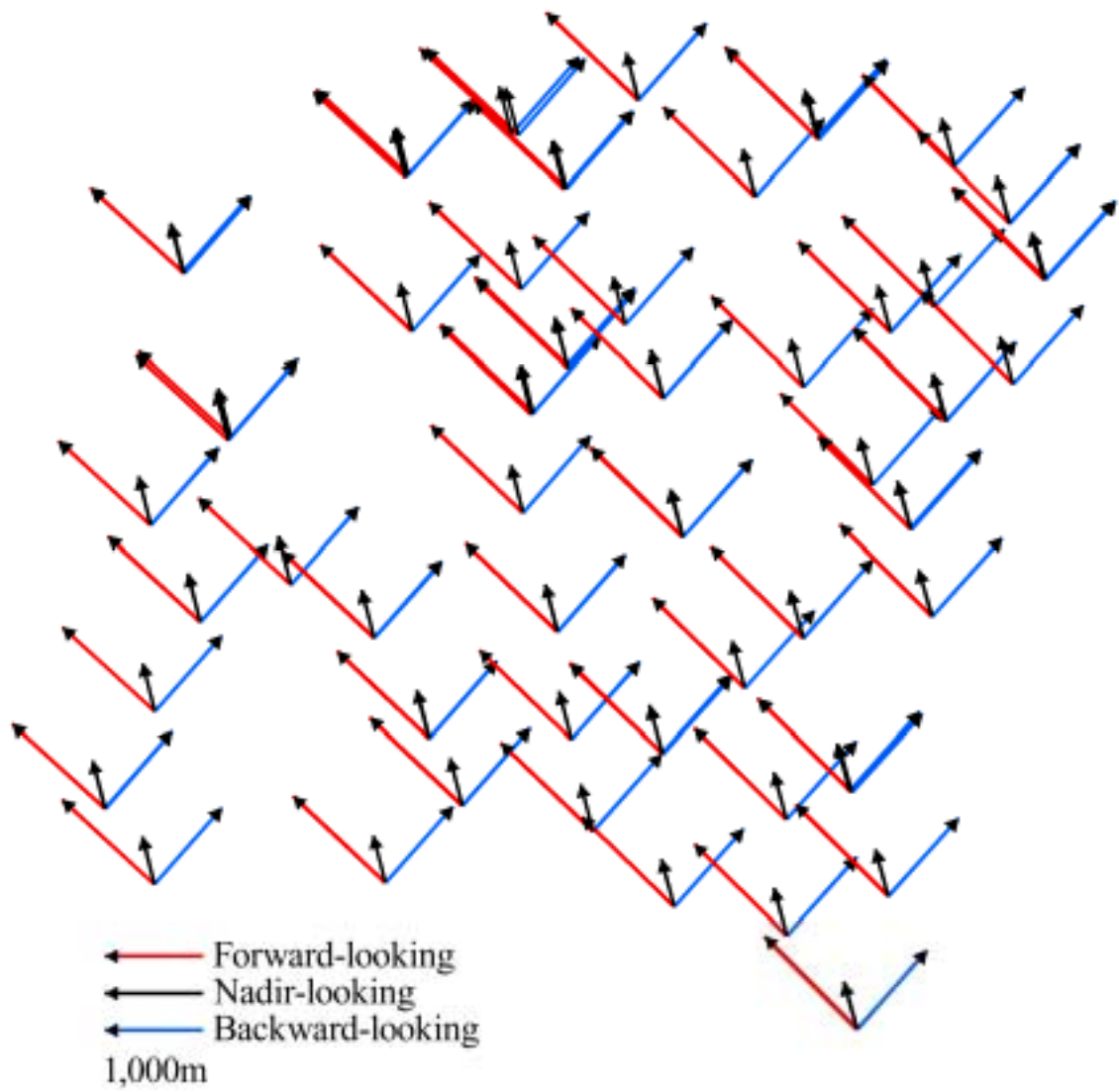
Fig. 4 Residuals of image observation (before the adjustment)
