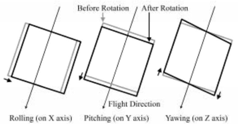
Fig. 6 Effect of radiometer rotation on ground space
